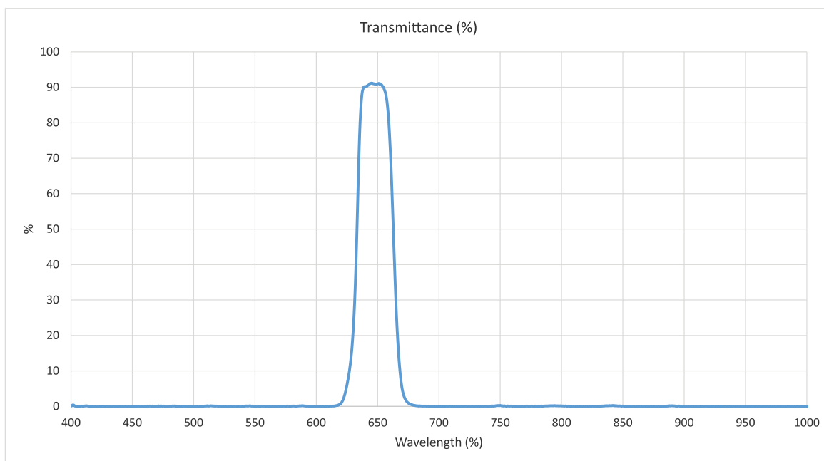
Image 12: Ambient light optical filter transmittance
