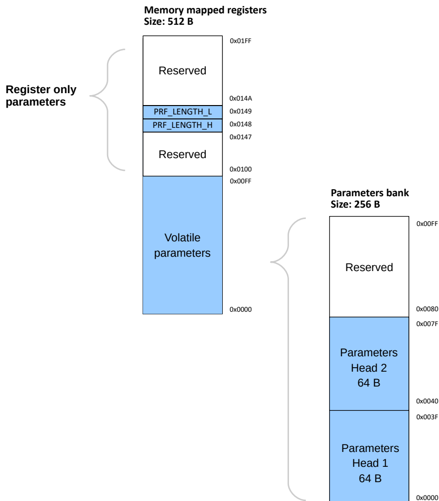
Image 11: Register map
