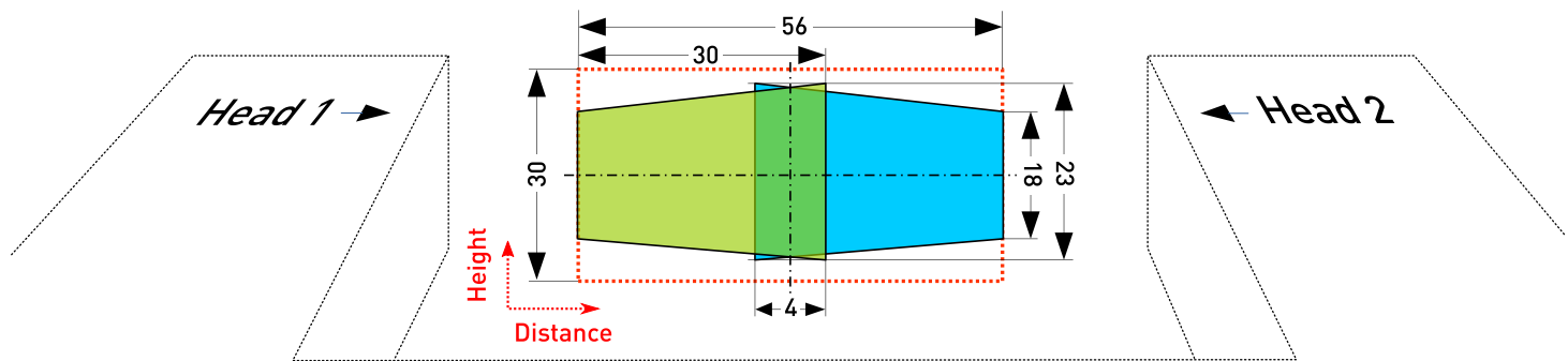
Image 4: Measuring range visualization
