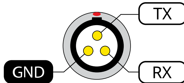
Image 2: I/O 1 connector (serial)
