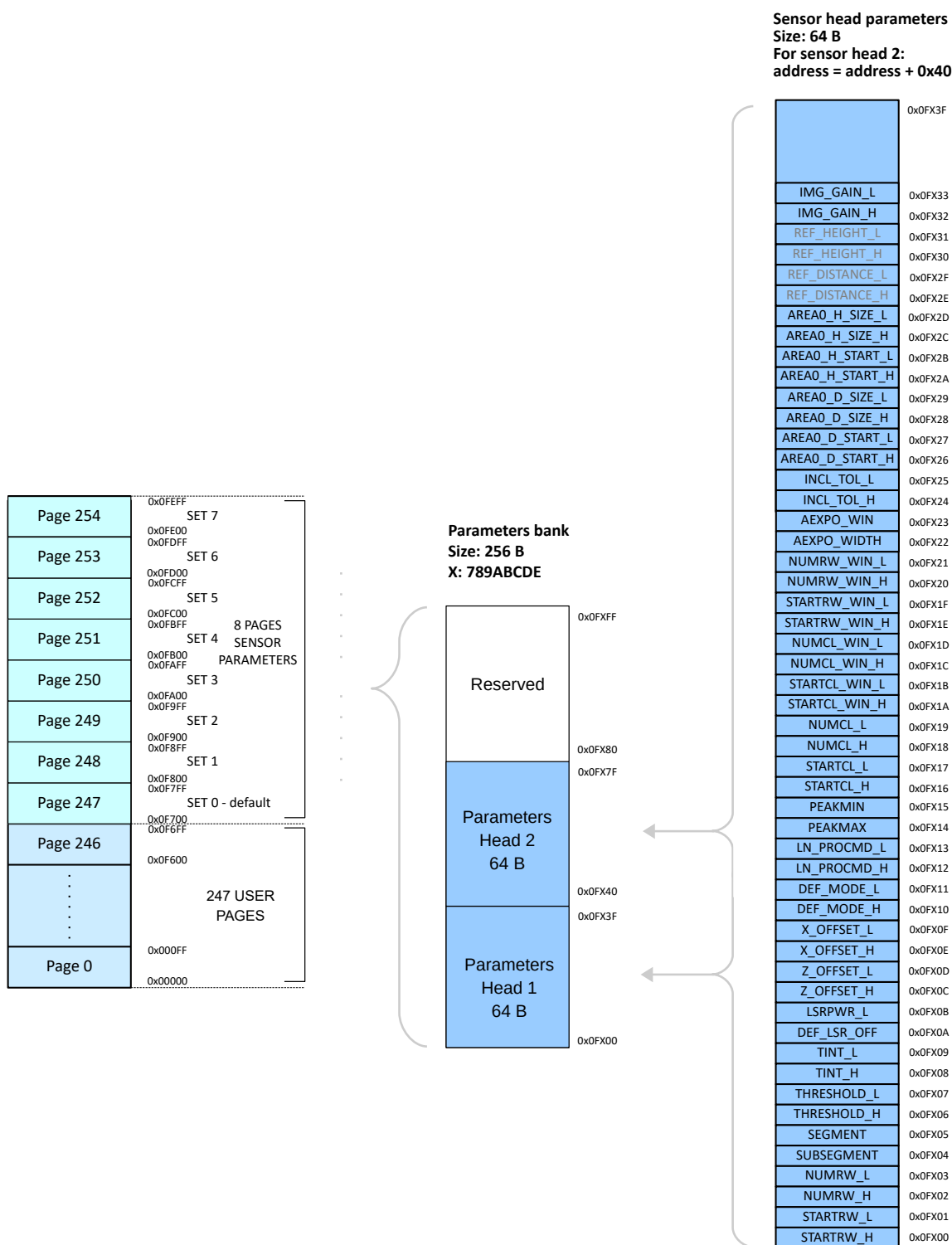
Image 10: Sensor memory structure
