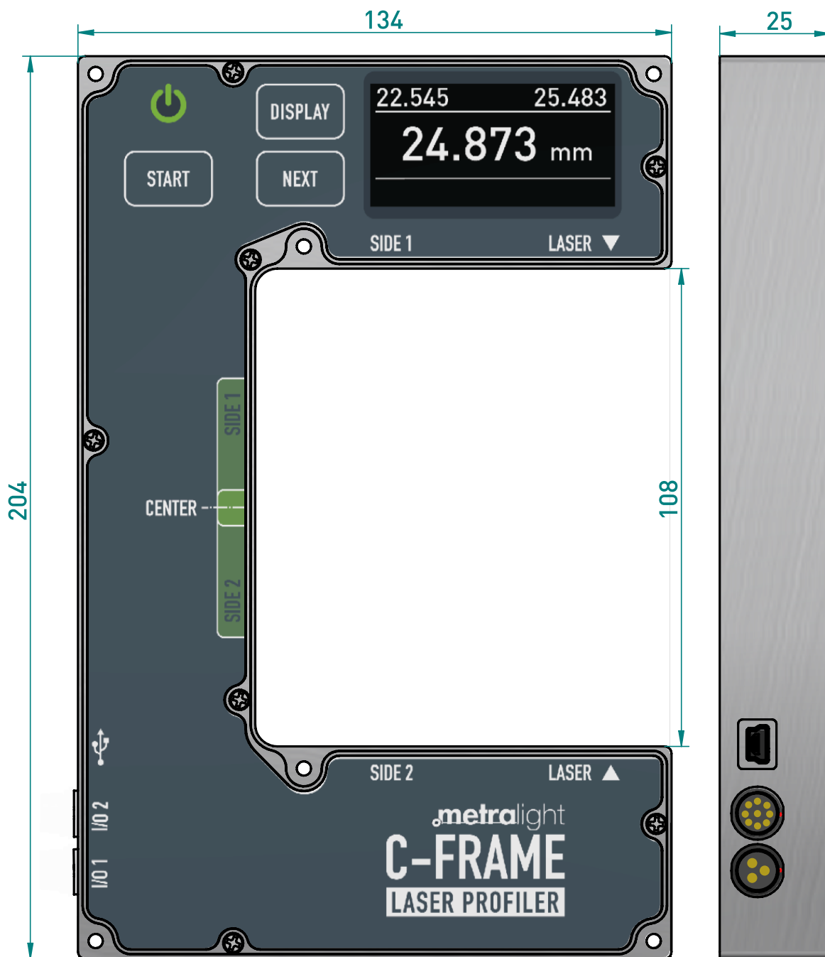
Image 1: C-frame sensor dimensions (mm)
