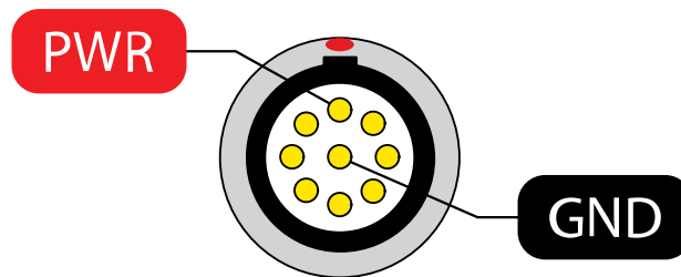
Image 3: I/O 2 connector (PWR)
